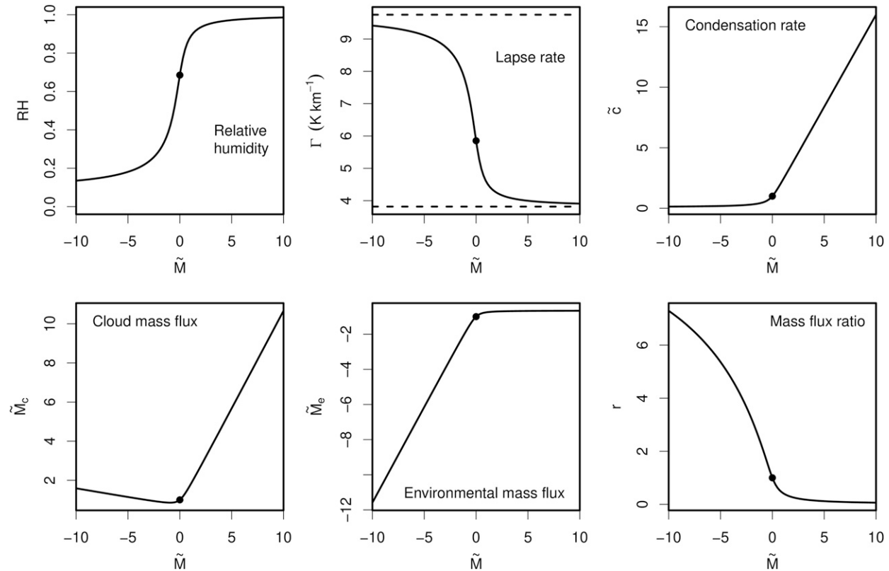
FIG. 2. Solutions from Eqs. (A37)–(A43) with p = 100 kPa, T = 300 K, and \varepsilon = \delta = 0.5 km ^{-1} . Circles denote values in RCE, i.e., at \tilde{M} = 0 . Dashed lines in the plot of lapse rate mark the moist and dry adiabats.
