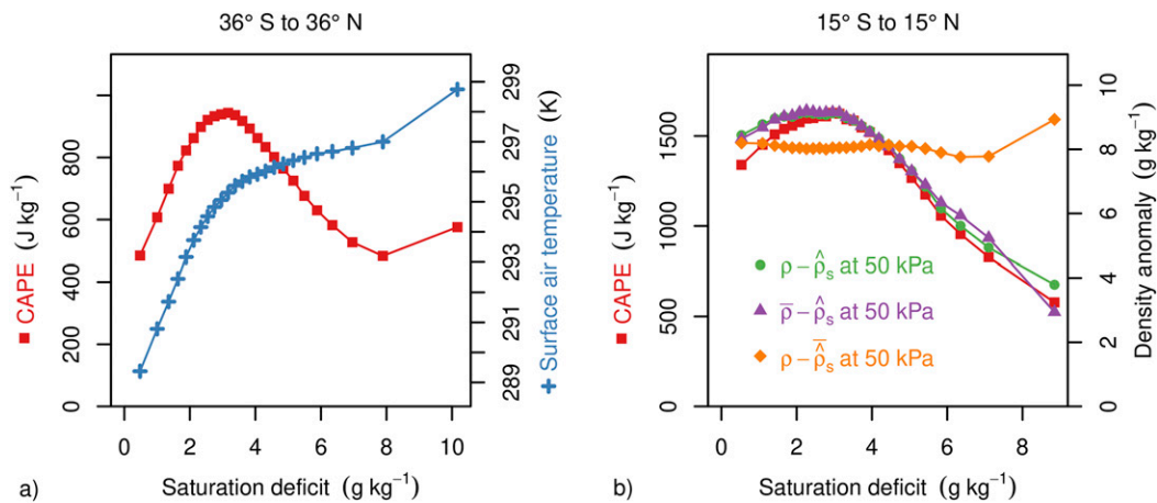
FIG. 4. (a) For soundings between 36^\circ\text{S} and 36^\circ\text{N} , conditionally averaged CAPE (red squares) and surface air temperature (blue plus signs) as functions of the lower-tropospheric saturation deficit. (b) For soundings between 15^\circ\text{S} and 15^\circ\text{N} , conditionally averaged CAPE (red squares), lifted-parcel density anomaly \rho - \hat{\rho}_s at 50 kPa (green circles), \bar{\rho} - \hat{\rho}_s at 50 kPa (purple triangles), and \rho - \bar{\rho}_s at 50 kPa (orange diamonds).
